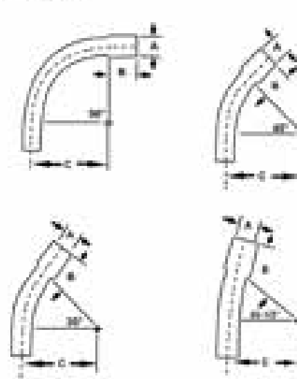
Bell End
